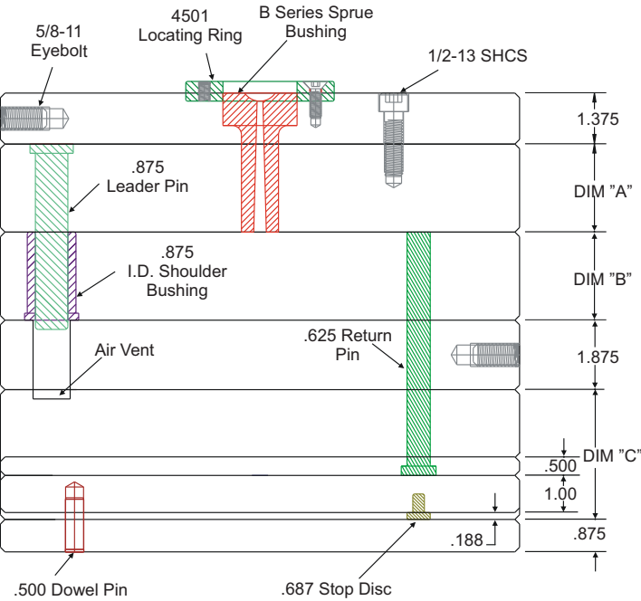
Section View
