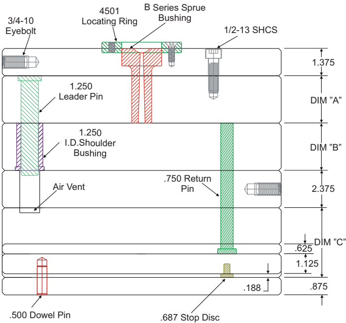
Section View
