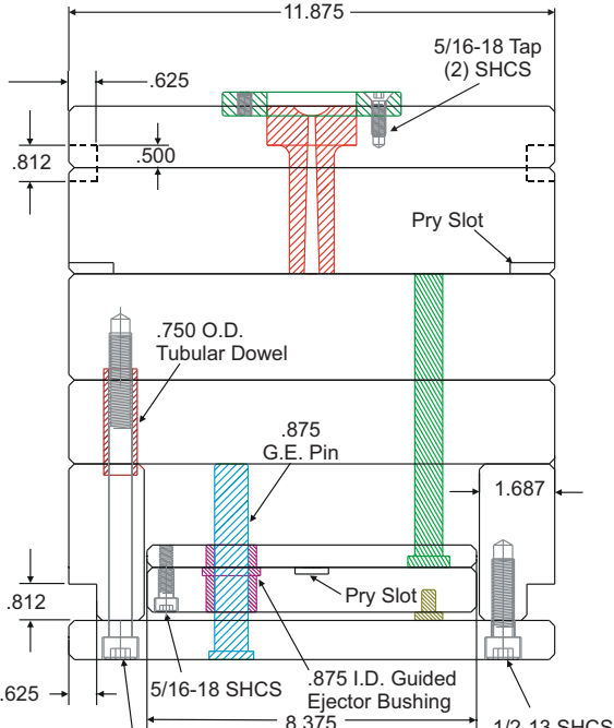
End View
