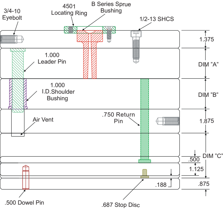
Section View
