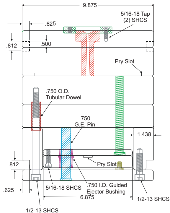
End View
